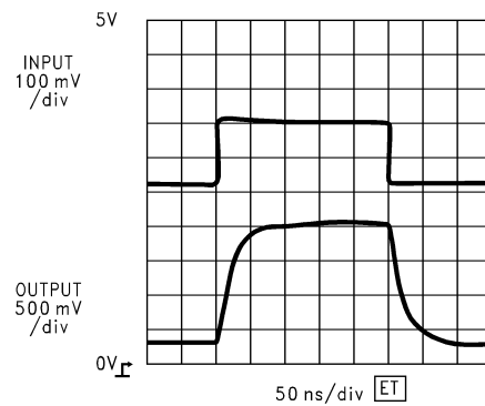
LM7131 Cable Driver A_V = +10 @ +5V
