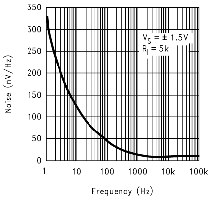
LM7131 Voltage Noise vs Frequency @ 3V
