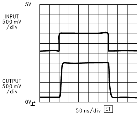
LM7131 Cable Driver A_V = +2 @ +5V
