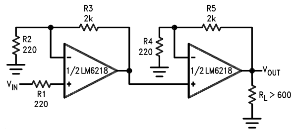
150 MHz Gain-Bandwidth Amplifier
