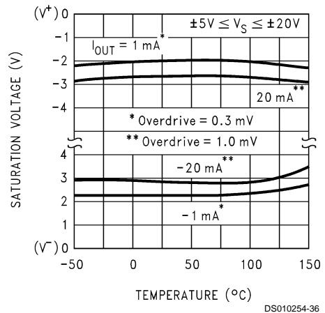
Output Saturation
