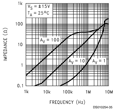
Output Impedance
