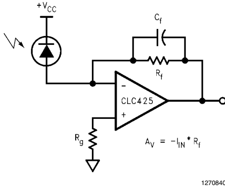
FIGURE 11. Transimpedance Amplifier Configuration
