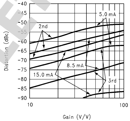
Distortion vs. Gain & I_{CC} ( V_{O1} = V_{PP} f_O = 3MHz )
