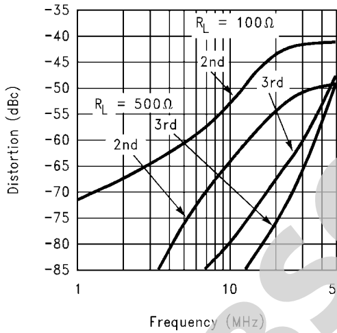
2nd and 3rd Harmonic Distortion ( V_{O1} = V_{PP} )
