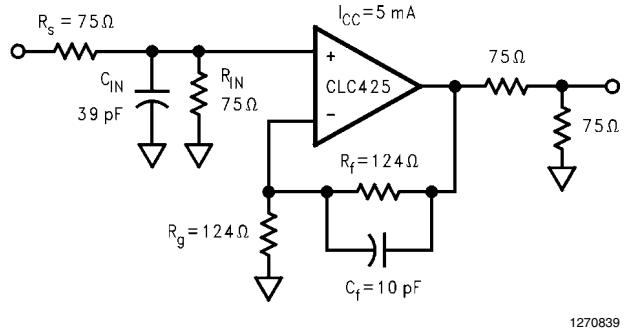
FIGURE 8. External Shunt Compensation
