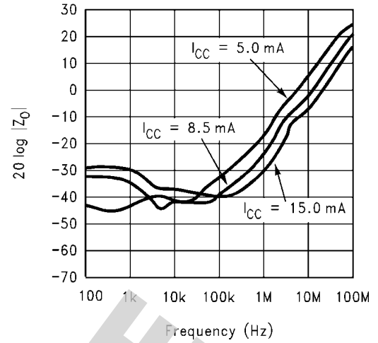
Closed-Loop Output Impedance
