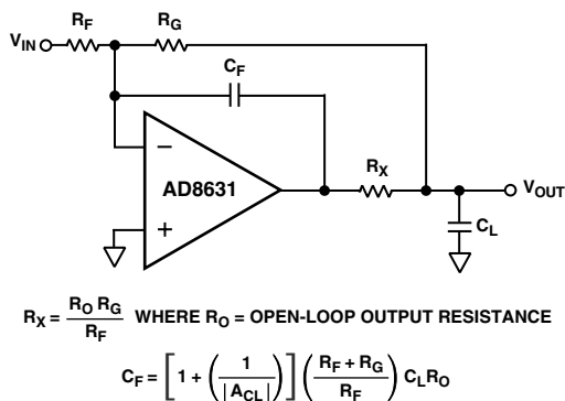
Figure 23. In-the-Loop Compensation Technique for Driving Capacitive Loads
