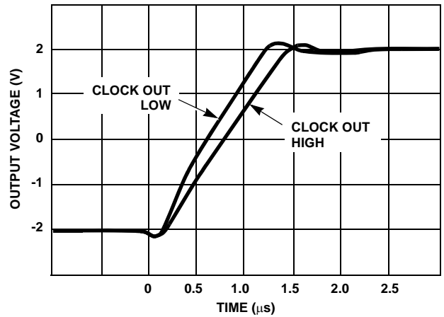
FIGURE 18. VOLTAGE FOLLOWER LARGE SIGNAL PULSE RESPONSE (NOTE)
