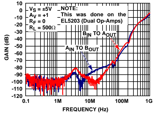
FIGURE 26. CHANNEL-TO-CHANNEL ISOLATION
