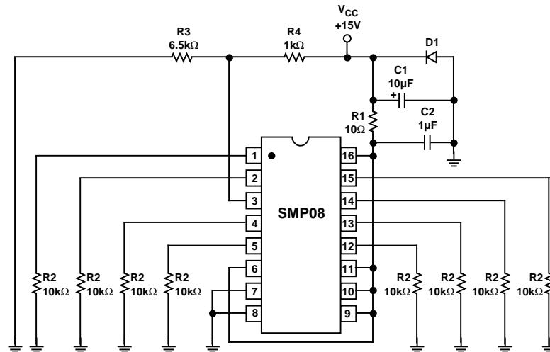
Figure 17. Burn-In Circuit
