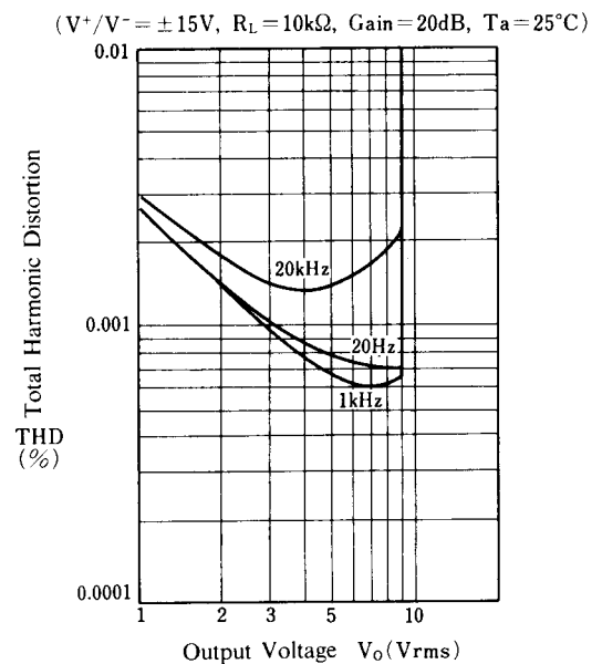
Total Harmonic distortion vs. Output Voltage
