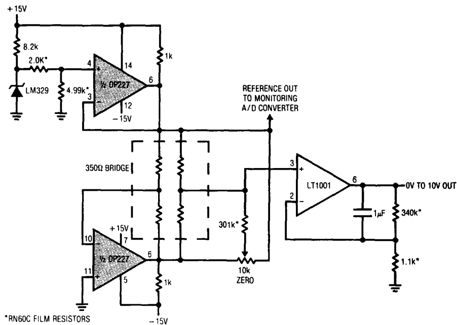
Strain Gauge Signal Conditioner with Bridge Excitation
