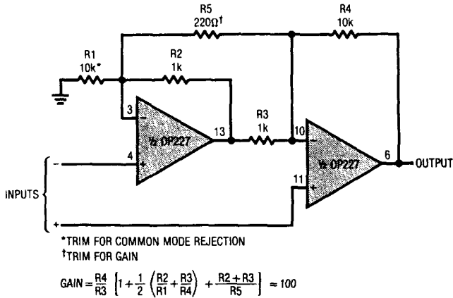
Two Op Amp Instrumentation Amplifier
