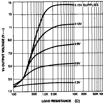
Figure 8. Negative Output Voltage Swing vs Load Resistance
