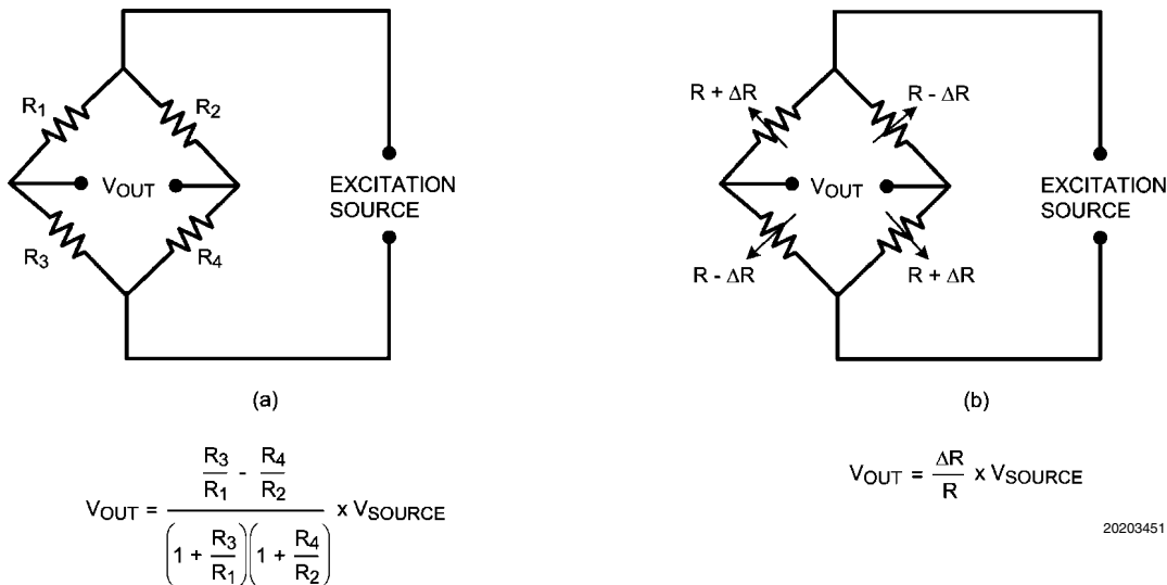
FIGURE 4. Bridge Sensor
