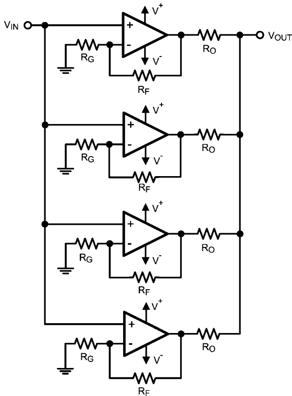
Figure 2 shows a schematic of this input voltage noise reduction circuit using the LMP2234. Typical resistor values are: R_G = 10\Omega , R_F = 1\text{ k}\Omega , and R_O = 1\text{ k}\Omega .
