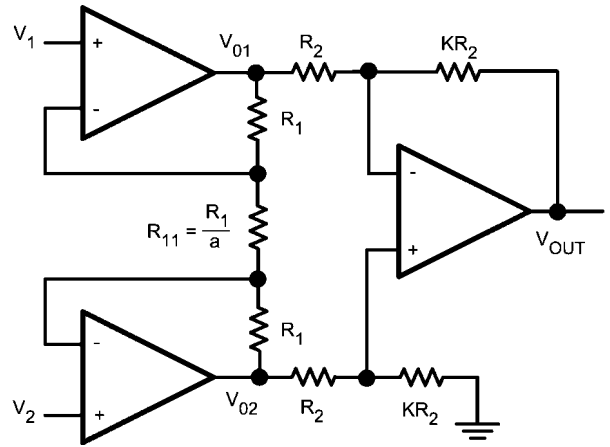
FIGURE 3. Instrumentation Amplifier
