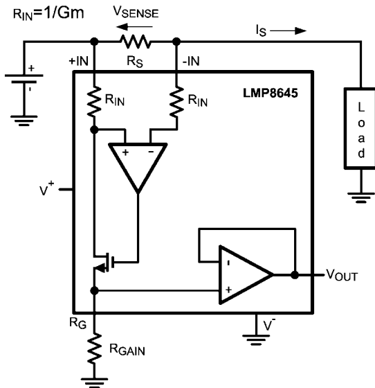
FIGURE 1. Current monitor
