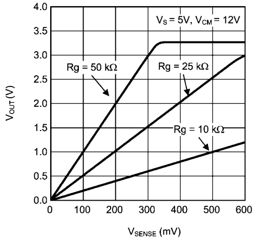
Output voltage vs. V_{SENSE}
