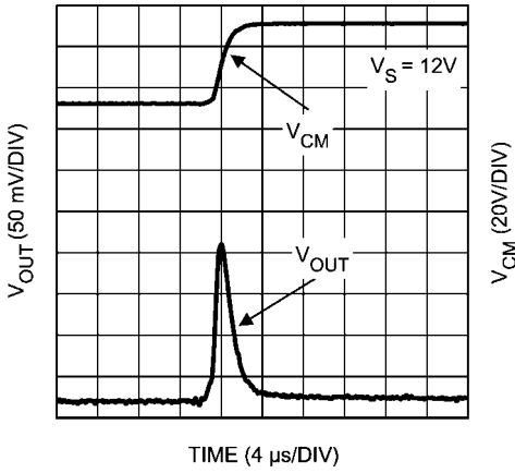
Common mode step response (rise)
