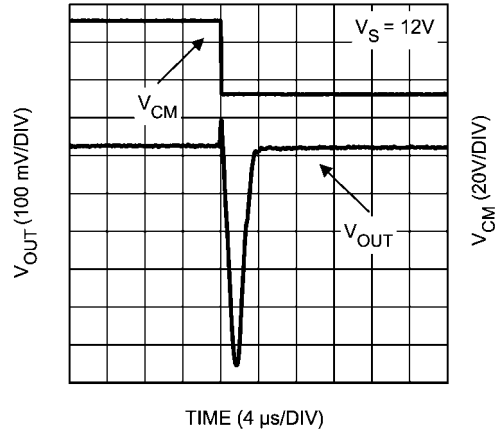
Common mode step response (fall)
