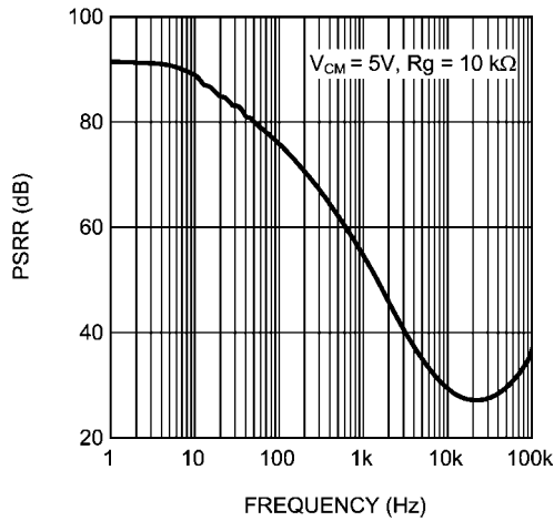
AC PSRR vs. Frequency
