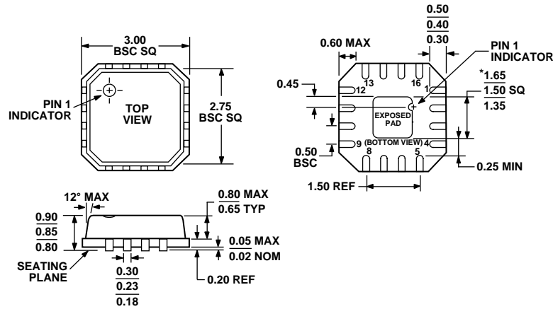
*COMPLIANT TO JEDEC STANDARDS MO-220-VEED-2 EXCEPT FOR EXPOSED PAD DIMENSION. Figure 42. 16-Lead Lead Frame Chip Scale Package [LFCSP_VQ] 3 mm × 3 mm Body, Very Thin Quad (CP-16-3) Dimensions shown in millimeters
