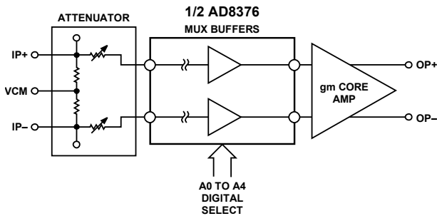
Figure 33. Simplified Schematic
