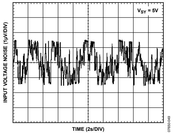
Figure 46. 0.1 Hz to 10 Hz Noise
