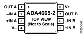
Figure 2. 8-Lead MSOP
