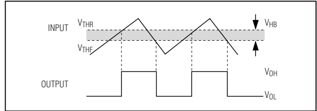
Figure 3. Hysteresis
