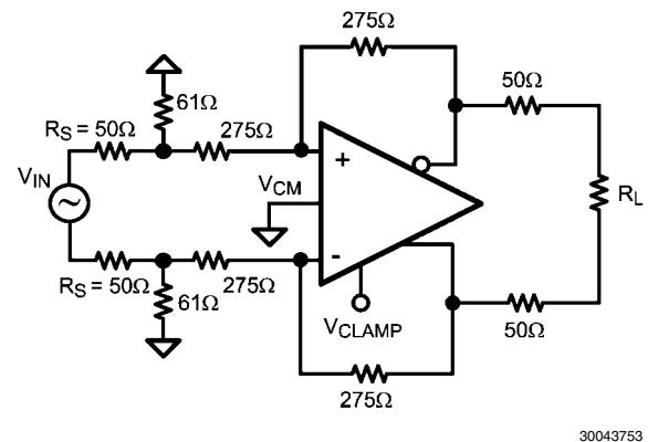
FIGURE 2. Differential S-Parameter Test Circuit
