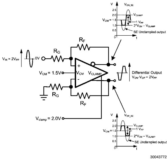
FIGURE 6. Clamp Operation
