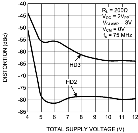
Distortion vs. Supply Voltage ( f_c=75MHz , R_L=200\Omega )
