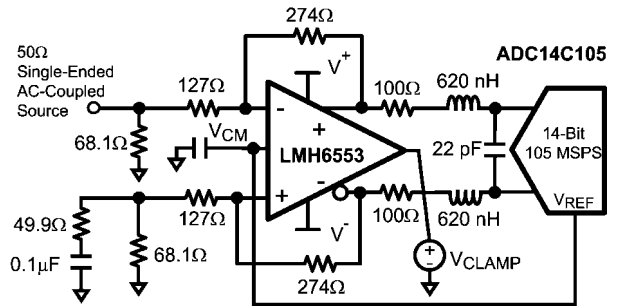
FIGURE 10. Driving a 14-bit ADC
