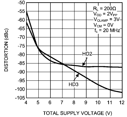
Distortion vs. Supply Voltage ( f_c=20MHz , R_L=200\Omega )
