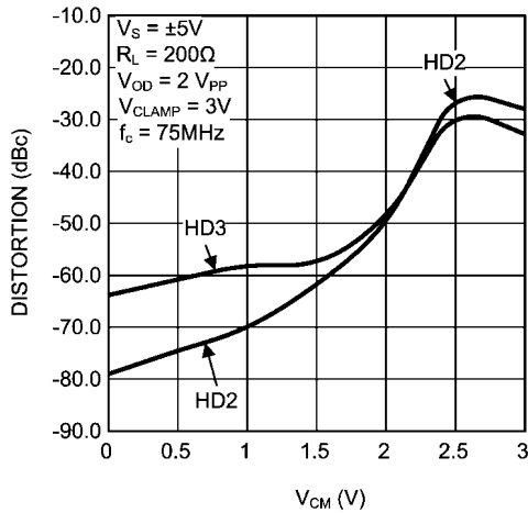
Distortion vs. V_{CM} ( f_c=75MHz , R_L=200\Omega )
