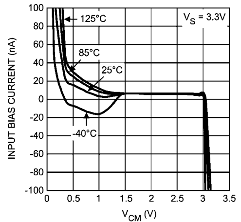
Input Bias Current vs. V_{CM}
