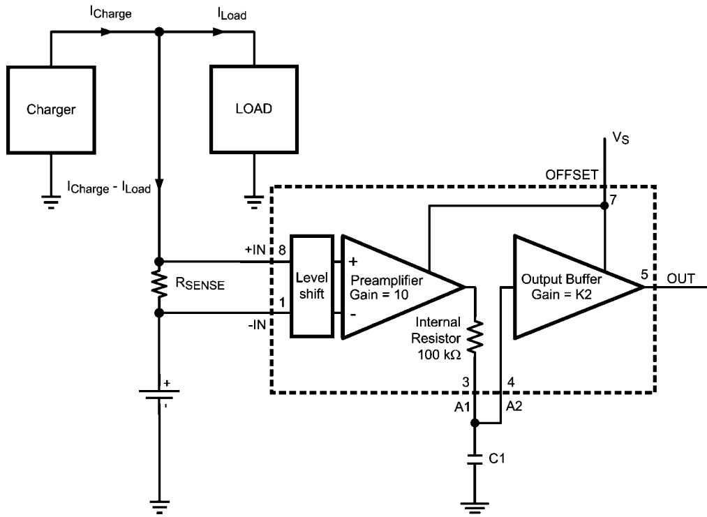
FIGURE 12. Battery Current Monitor Application
