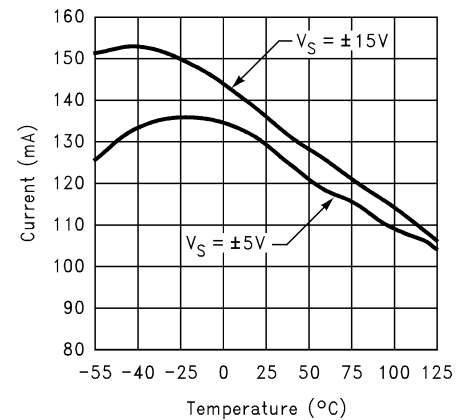
Short Circuit Current vs. Temperature (Sourcing)
