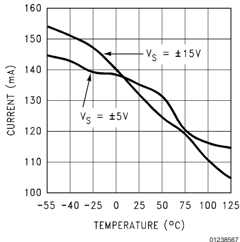
Short Circuit Current vs. Temperature (Sourcing)
