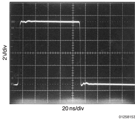
FIGURE 6. Properly Terminated Signal
