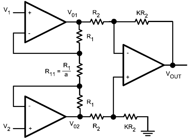
FIGURE 3. Instrumentation Amplifier
