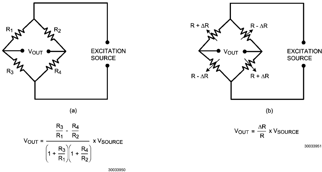
FIGURE 4. Bridge Sensor
