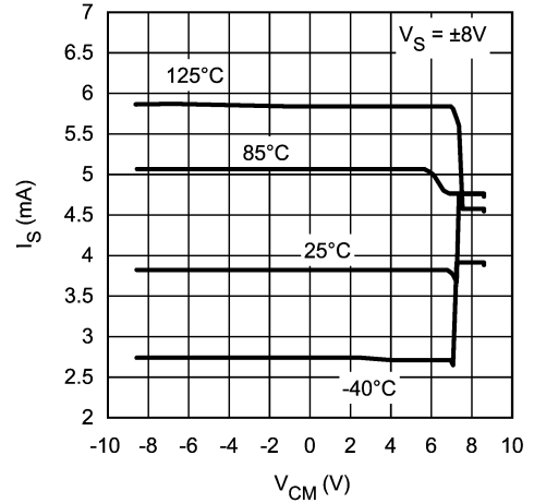
I_S vs. V_{CM} for Various Temperature
