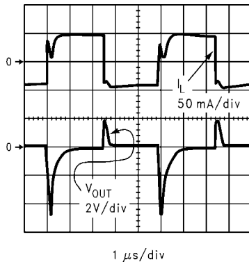
FIGURE 9. V COM driver performance scope photo
