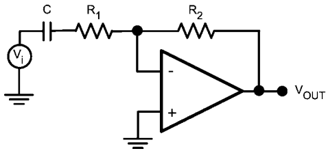
FIGURE 5. Highpass Filter
