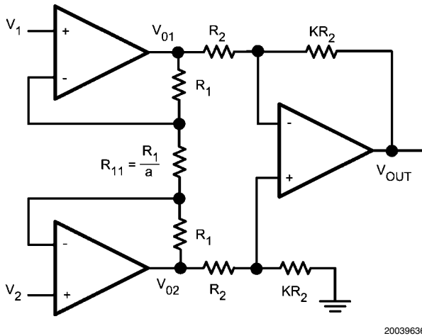
FIGURE 1. Instrumentation Amplifier
