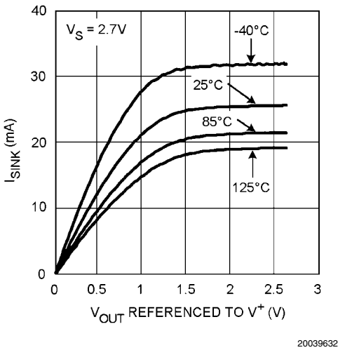
Sinking Current vs. V OUT (Note 14)
