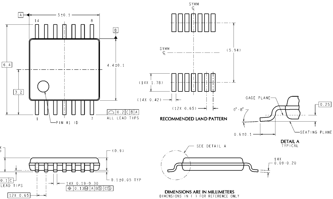
14-Pin TSSOP NS Package Number MTC14
