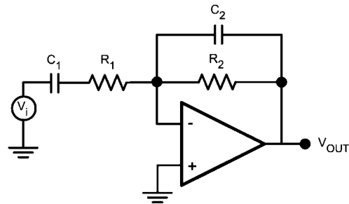
FIGURE 7. Bandpass Filter
