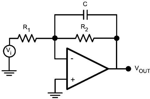
FIGURE 3. Lowpass Filter
