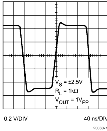
Large Signal Step Response
