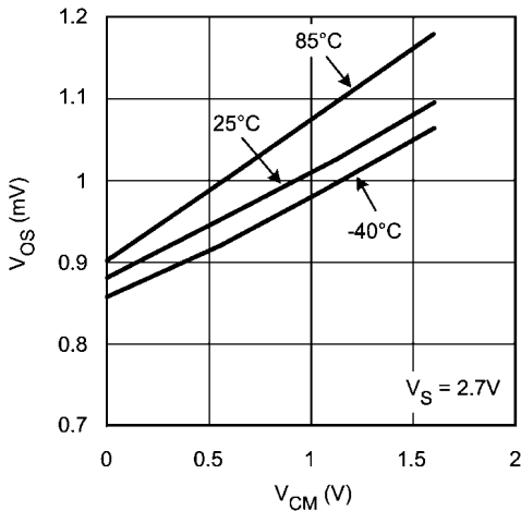
Offset Voltage vs. Common Mode Voltage (A Typical Unit)
