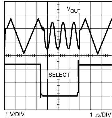
FIGURE 5. 2:1 MUX Output
