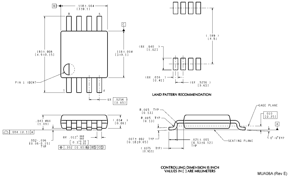
DIMENSIONS ARE IN MILLIMETERS DIMENSIONS IN ( ) FOR REFERENCE ONLY 6-Pin SC70 NS Package Number MAA06A
