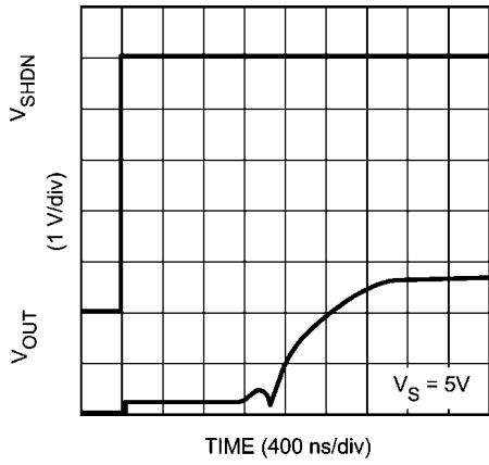
FIGURE 3. Turn-on Time
