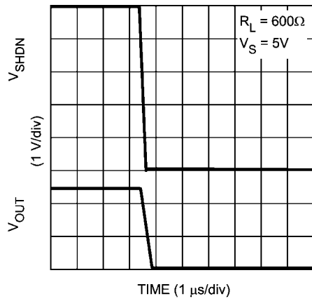
FIGURE 4. Turn-off Time
