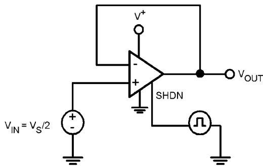
FIGURE 5. Turn-on Time
