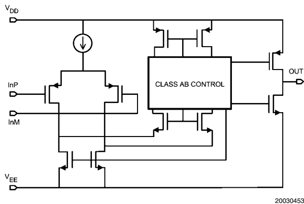
FIGURE 1. Simplified Schematic
