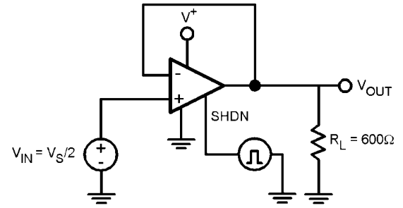
FIGURE 6. Turn-off Time
