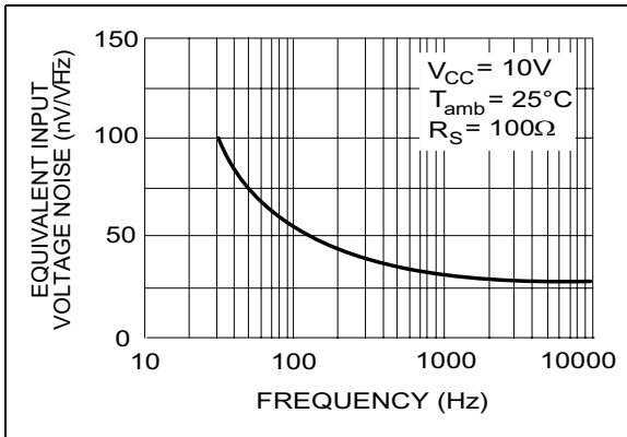
Figure 14. Input voltage noise vs. frequency
