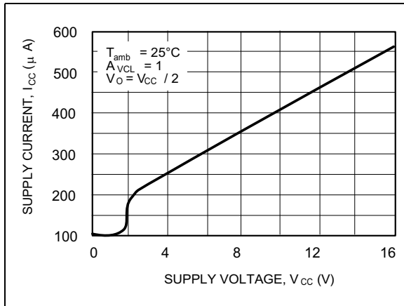
Figure 2. Supply current (each amplifier) vs. supply voltage
