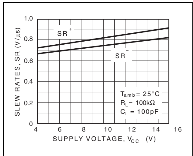
Figure 28. Slew rate versus supply voltage
