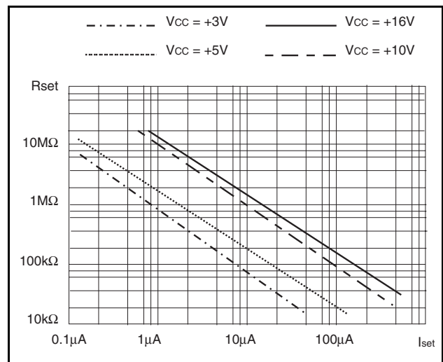
Figure 6. Rset connected to Vcc-
