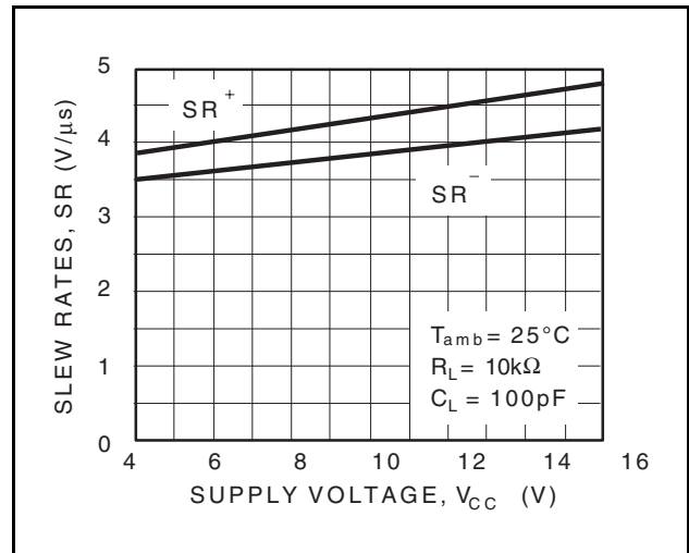
Figure 39. Slew rate versus supply voltage
