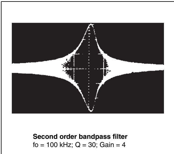
Figure 23. Output A
