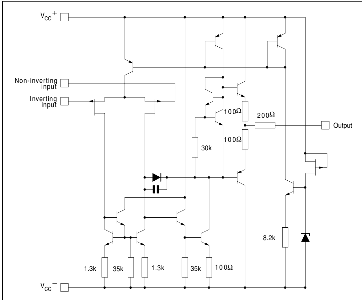
Figure 1. Circuit schematics (for each amplifier)
