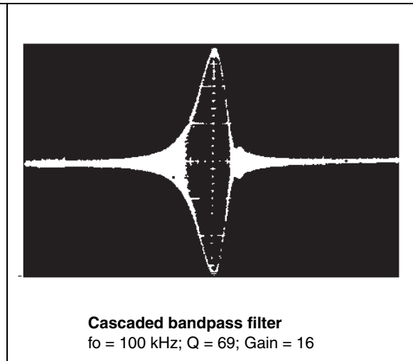
Figure 24. Output B
