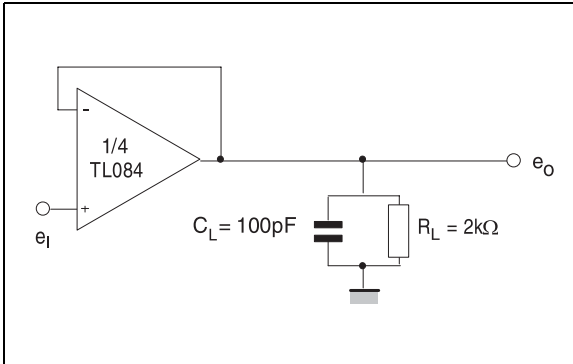
Figure 19. Voltage follower
