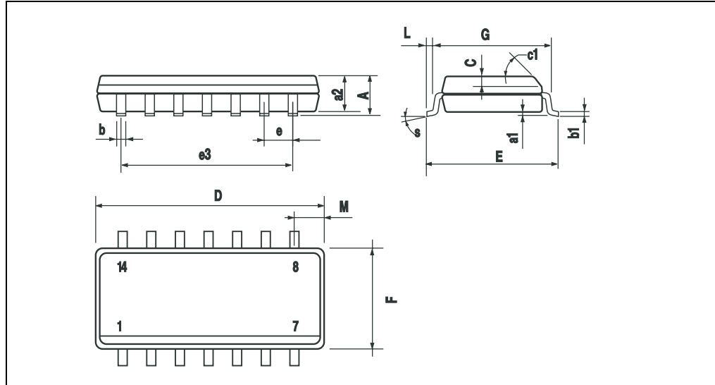
Figure 28. SO-14 package mechanical drawing
