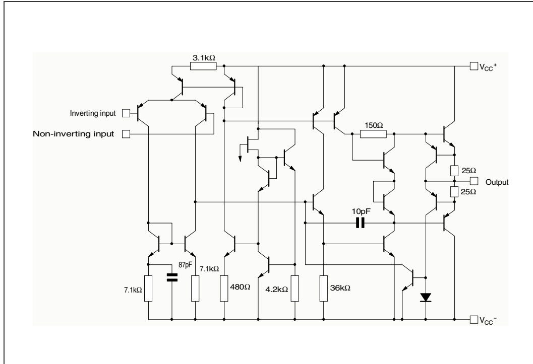
Figure 1. Schematic diagram (1/2MC4558)
