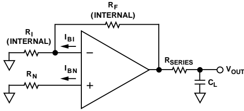
Figure 24. Output Offset Voltage
