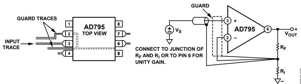
Figure 35. Guard Scheme—Follower
