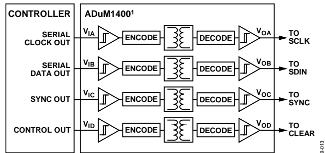
Figure 57. Isolated Interface
