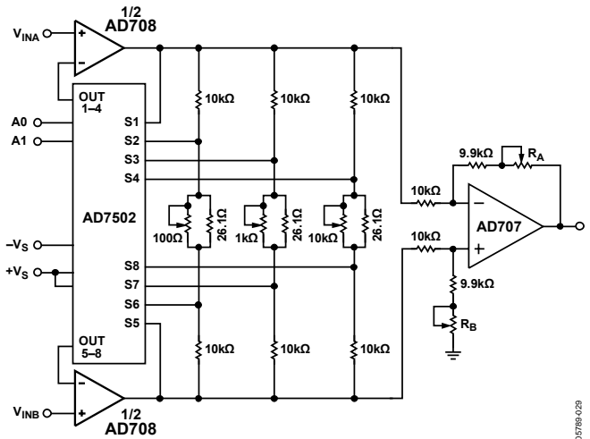
Figure 29. Precision PGA
