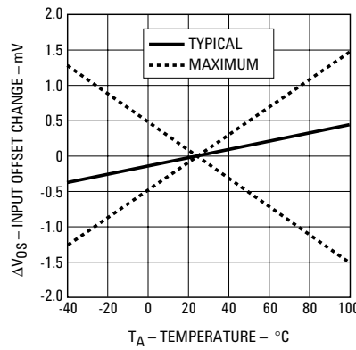
Figure 7. Input offset change vs. temperature.
