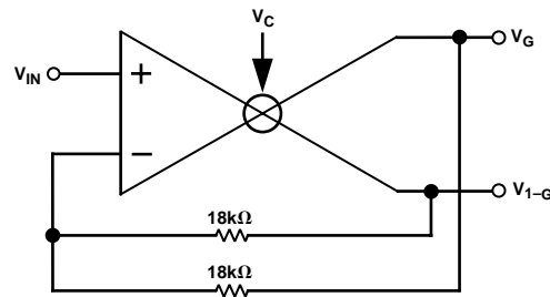
Figure 9. Basic VCP Connection
