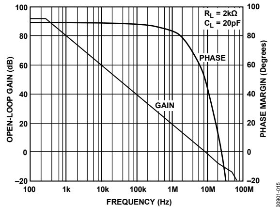
Figure 15. Open-Loop Gain and Phase Margin vs. Frequency
