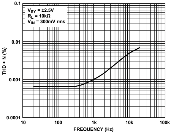
Figure 51. THD + Noise vs. Frequency
