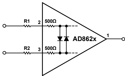
Figure 54. Input Protection
