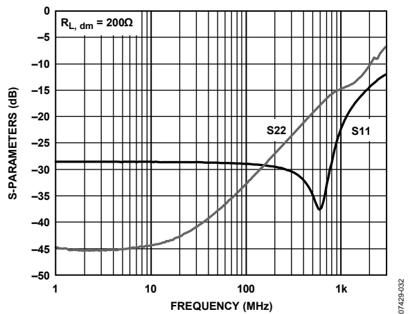
Figure 27. Return Loss (S11, S22) vs. Frequency
