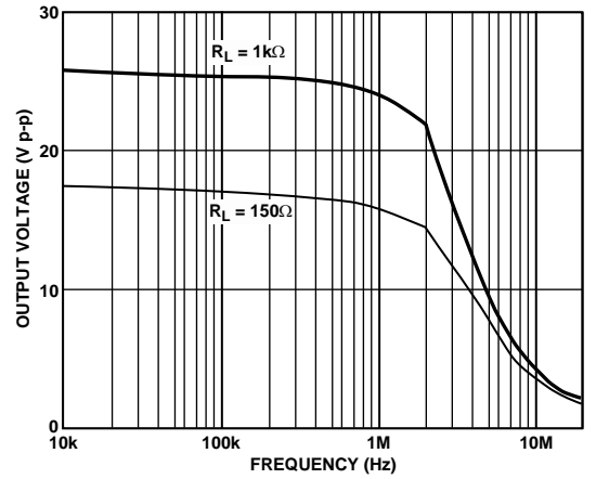
Figure 16. Large Signal Frequency Response; G = +2
