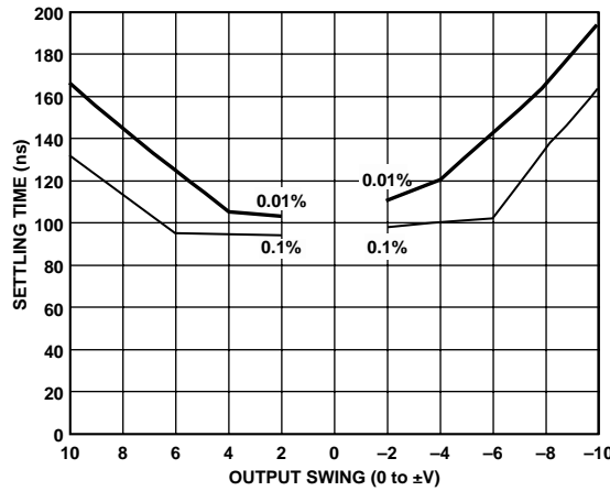
Figure 17. Output Swing and Error vs. Settling Time
