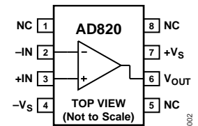
Figure 2. 8-Lead SOIC_N and 8-Lead MSOP
