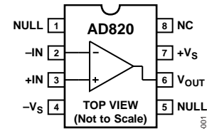
Figure 1. 8-Lead PDIP
