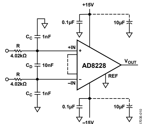
Figure 47. RFI Suppression
