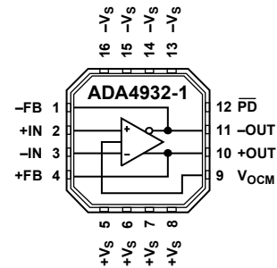
Figure 1. ADA4932-1
