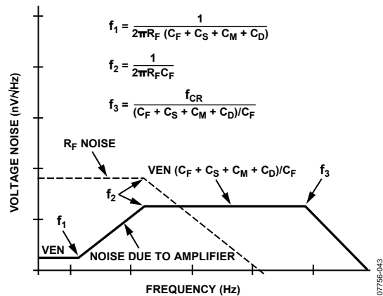
Figure 45. Photodiode Voltage Noise Contributions
