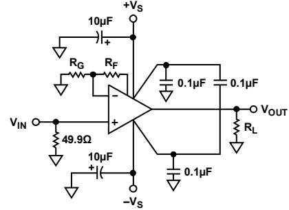
Figure 35. Noninverting Gain Configuration
