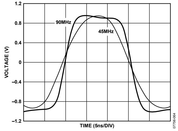
Figure 51. Large Signal Transient Response (Low-Pass Filter)
