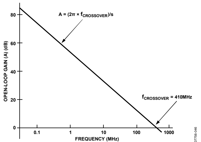
Figure 40. Open-Loop Gain vs. Frequency and Basic Connections
