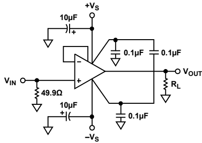
Figure 32. G = 1 Configuration
