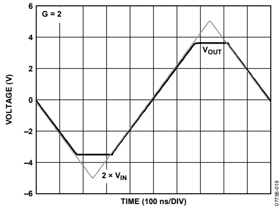
Figure 19. Output Overdrive Recovery
