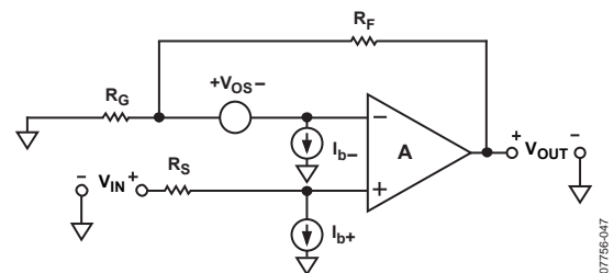
Figure 41. Voltage Feedback Amplifier's DC Errors
