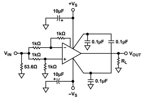
Figure 37. Common-Mode Rejection
