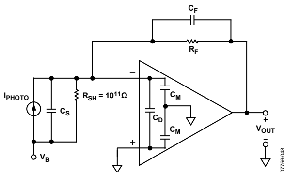
Figure 44. Wideband Photodiode Preamp
