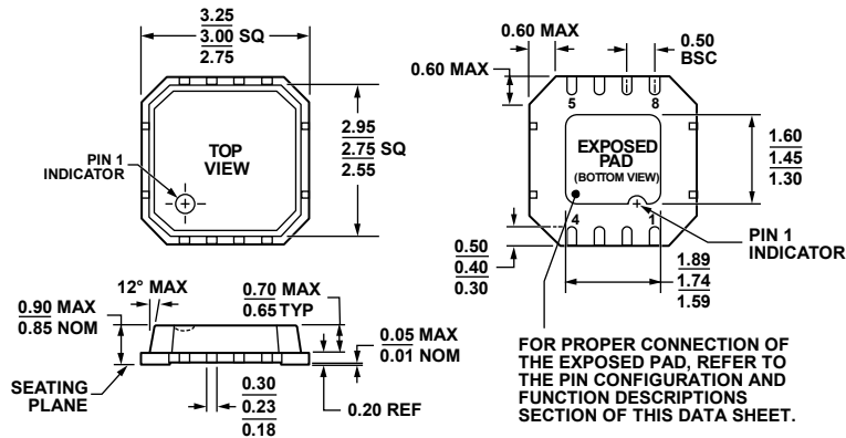
Figure 52. 8-Lead Lead Frame Chip Scale Package [LFCSP_VD] 3 mm × 3 mm Body, Very Thin, Dual Lead (CP-8-2) Dimensions shown in millimeters
