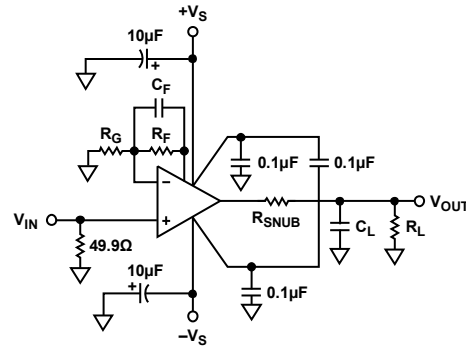
Figure 42. R_{SNUB} or C_F Used to Reduce Peaking
