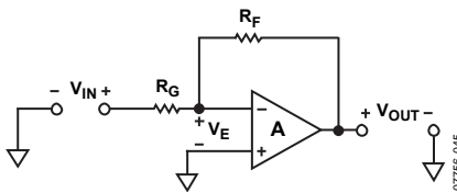
Figure 39. Inverting Configuration
