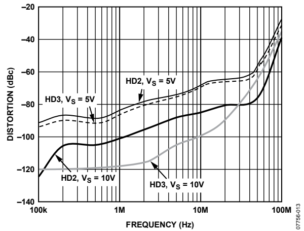
Figure 16. Distortion vs. Frequency for Various Supplies, V_{OUT} = 2 \text{ V p-p}
