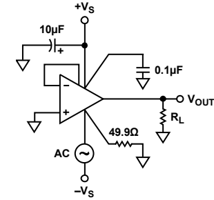
Figure 36. Negative Power Supply Rejection
