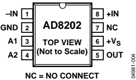
Figure 4. Pin Configuration
