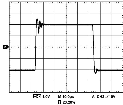
Figure 38. Large Signal Response, C_L = 5 nF
