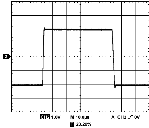
Figure 37. Large Signal Response, C_L = 0 pF
