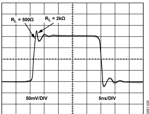
Figure 26. Small Signal Transient Response for Various R_L , V_S = \pm 5 V
