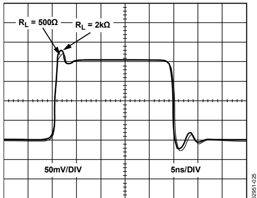
Figure 25. Small Signal Transient Response for Various R_L , V_S = 5 V
