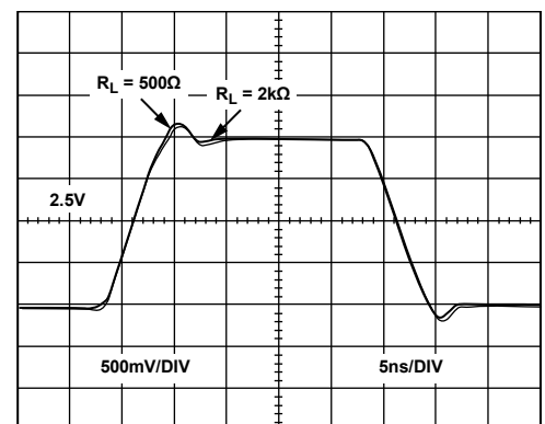
Figure 29. Large Signal Transient Response for Various R_L , V_S = 5 V
